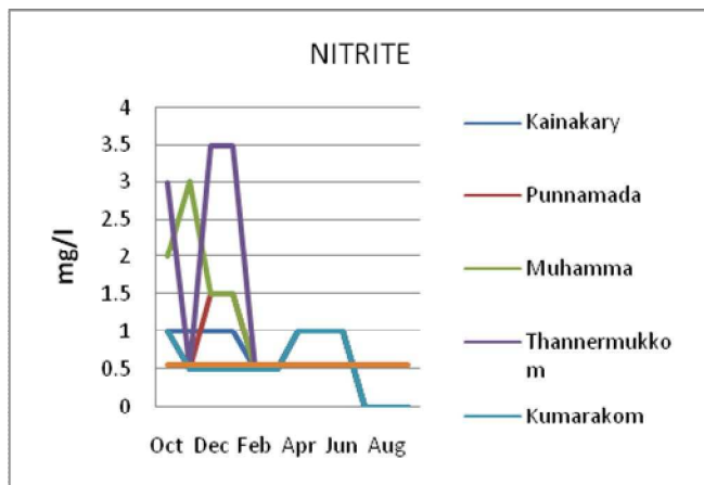
Figure.3 Nitrate level in Vembanad lake (October 2009- September 2010)
