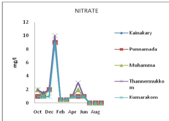
Figure 2 . Nitrate levels in Vembanad lake (October 2009 to September 2010)
