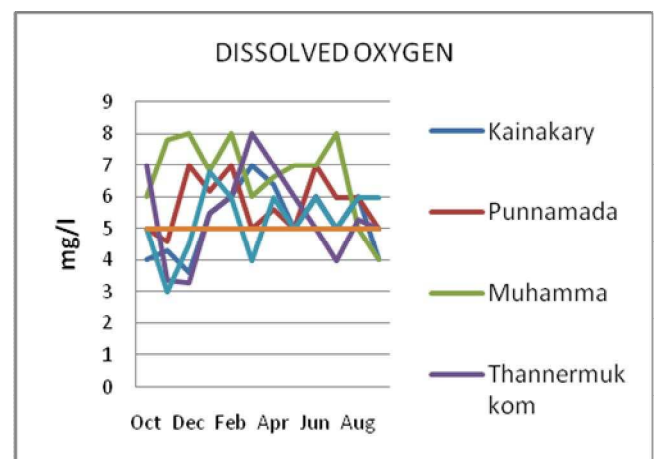
Figure 6 . DO levels in Vembanad lake (October 2009 to September 2010)
