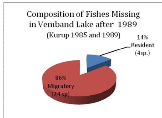
Figure 8. Composition of fishes missing in Vembanad Lake after 1989
