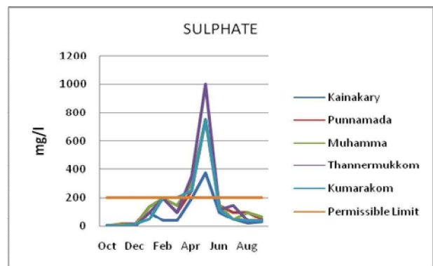
Figure 5 . Sulphate levels in Vembanad lake (October 2009 to September 2010)
