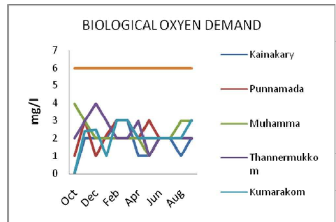
Figure 7. BOD levels in Vembanad lake (October 2009 to September 2010)
