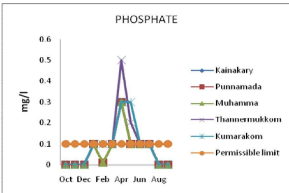
Figure 4 . Phosphate levels in Vembanad lake (October 2009 to September 2010)
