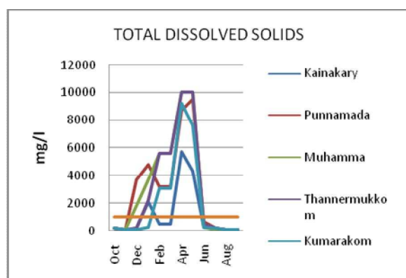
Figure 1 . TDS levels in Vembanad lake (October 2009 to September 2010)
